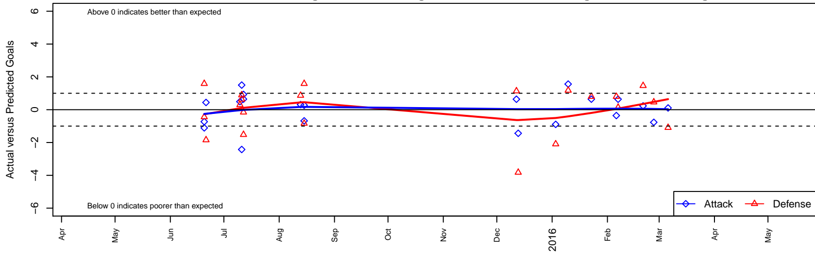
Snohomish United Red G97 Dots are actual minus expected GF (blue circles) and GA (red triangles). Blue line is smoothed change in attack strength. Red is smoothed change in defense strength.
